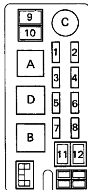
Relay Block No. 2
